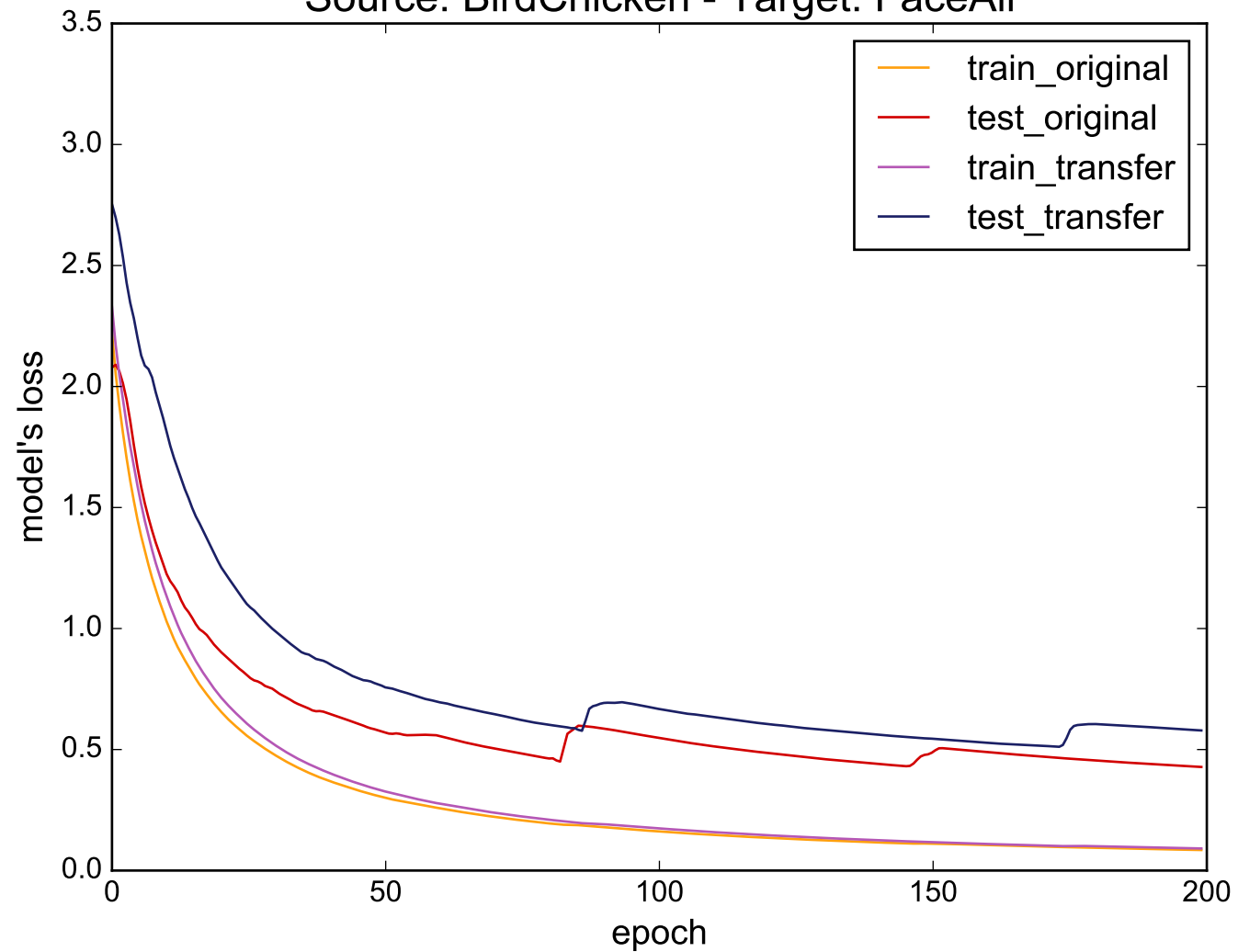
Source: BirdChicken - Target: FaceAll
