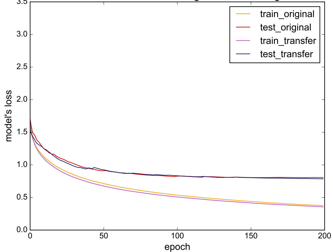
Source: BirdChicken - Target: MedicalImages
