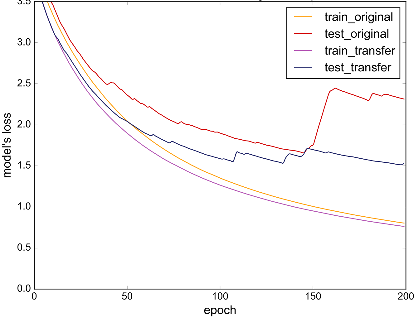
Source: BirdChicken - Target: ShapesAll
