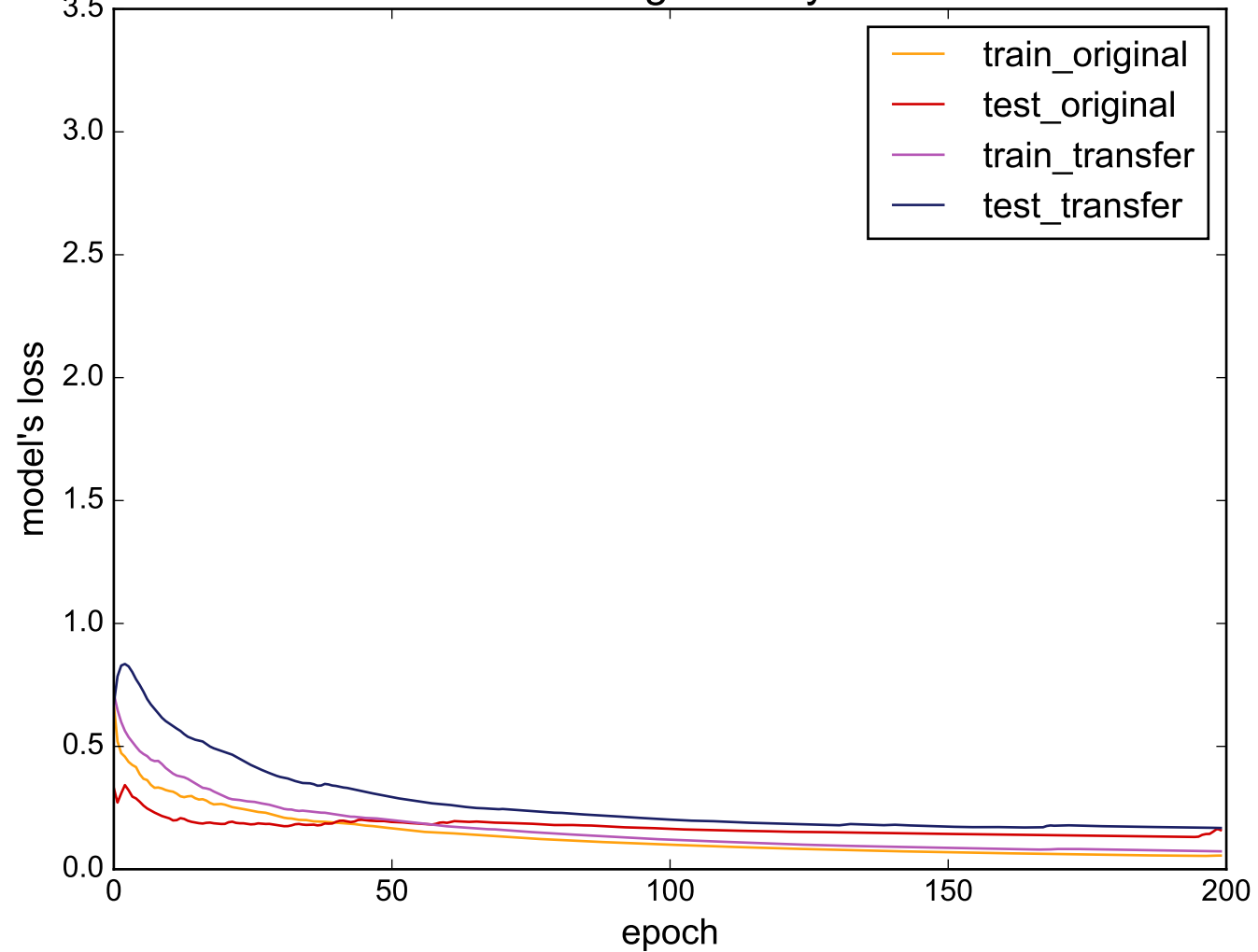
Source: BirdChicken - Target: SonyAIBORobotSurface
