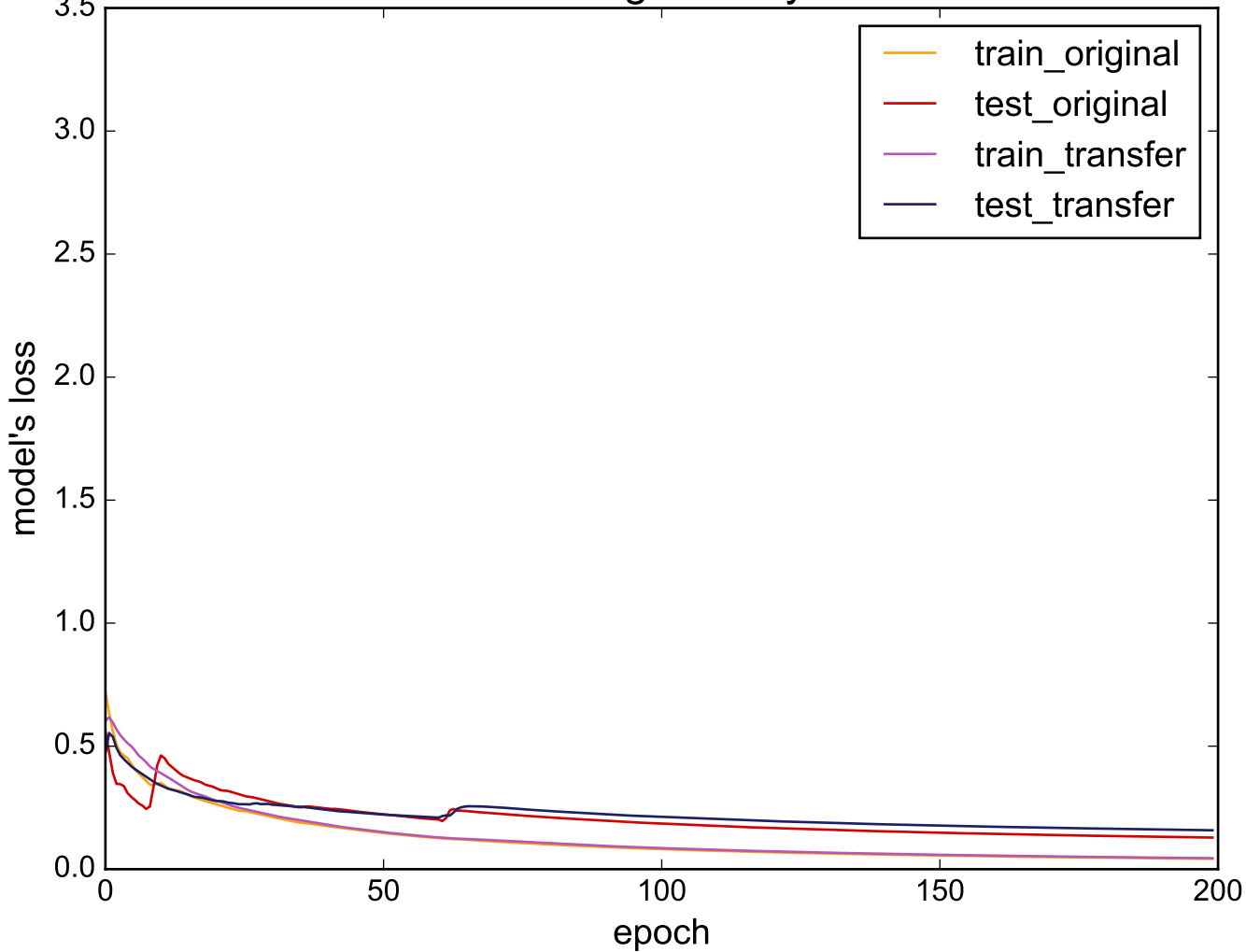
Source: BirdChicken - Target: SonyAIBORobotSurfaceII
