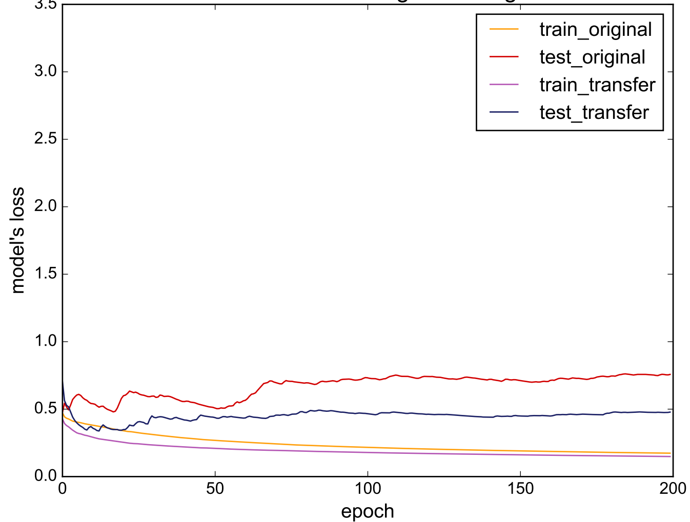
Source: BirdChicken - Target: StarLightCurves
