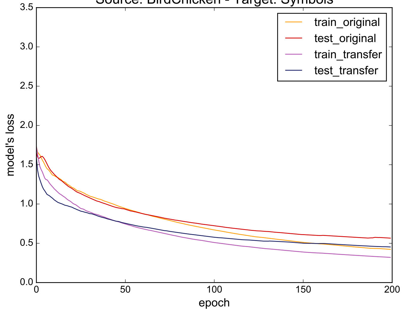
Source: BirdChicken - Target: Symbols
