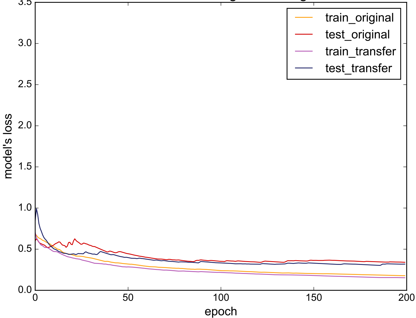
Source: BirdChicken - Target: ToeSegmentation1
