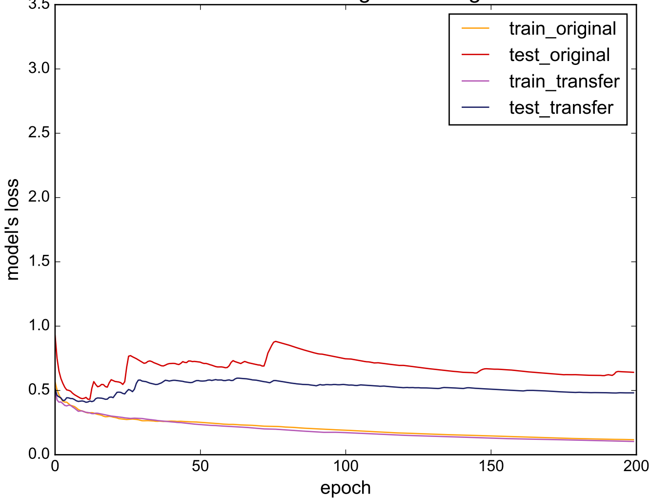
Source: BirdChicken - Target: ToeSegmentation2
