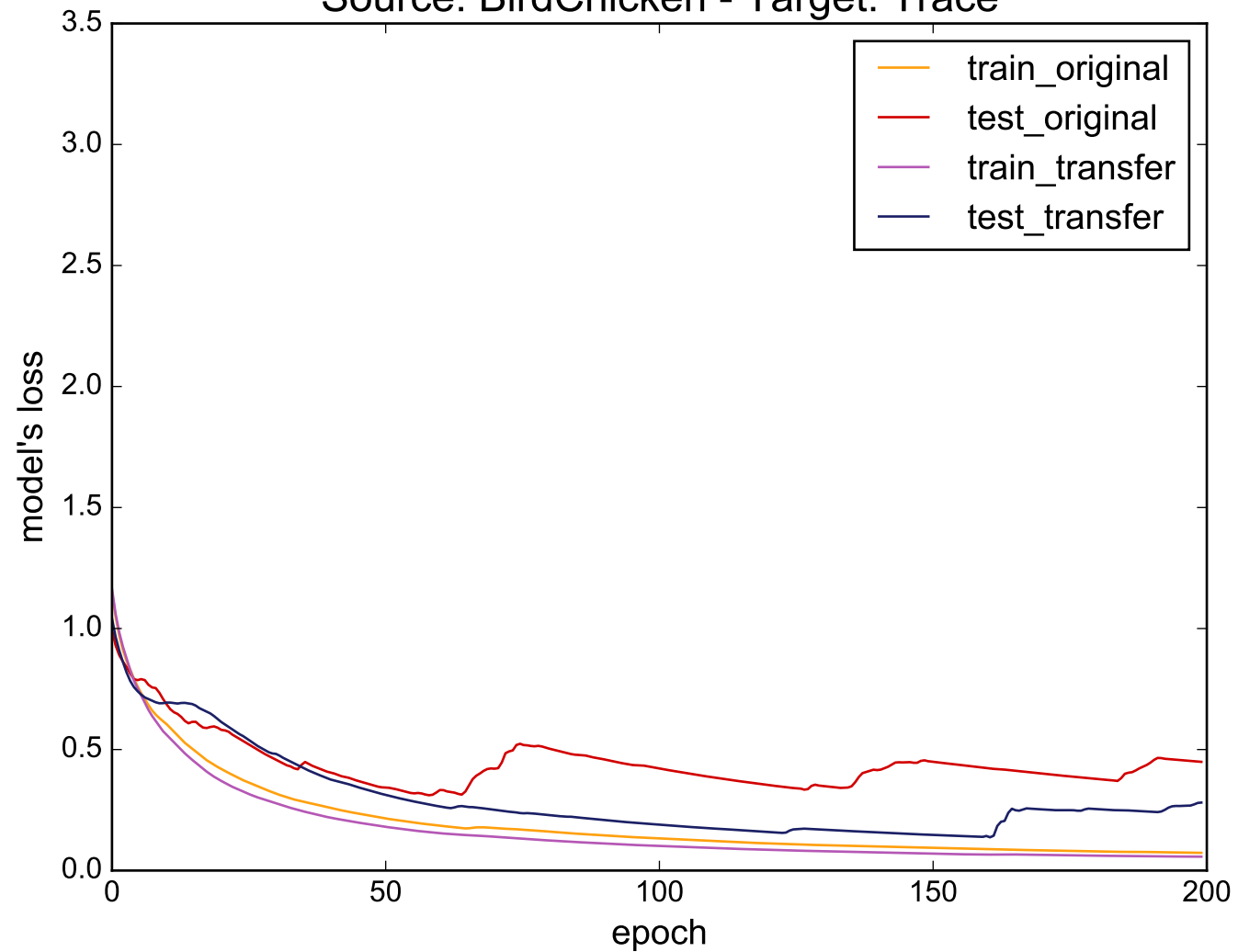
Source: BirdChicken - Target: Trace
