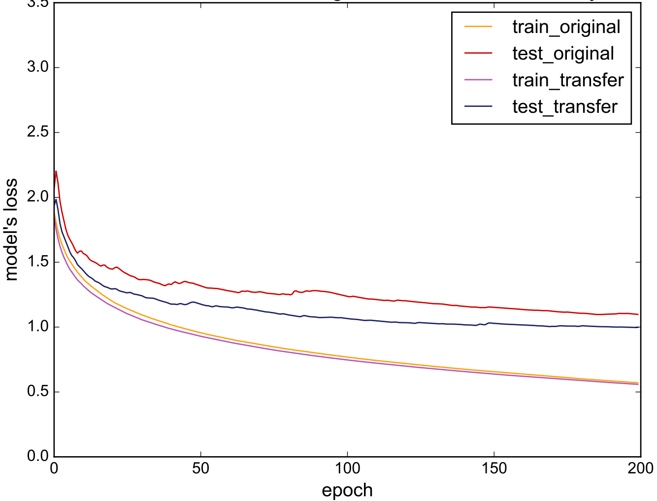
Source: BirdChicken - Target: UWaveGestureLibraryAll
