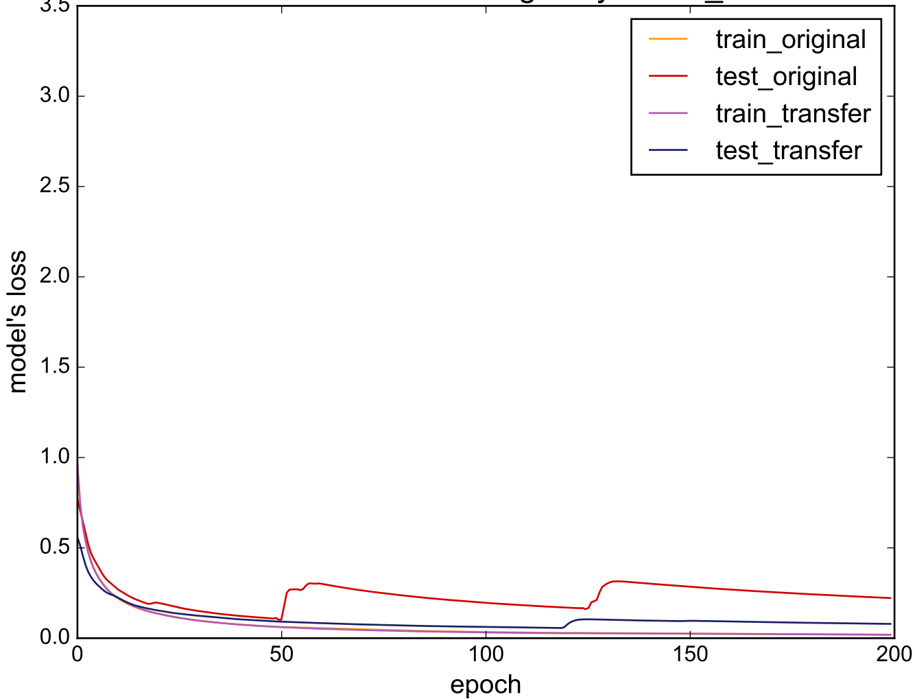
Source: BirdChicken - Target: synthetic_control
