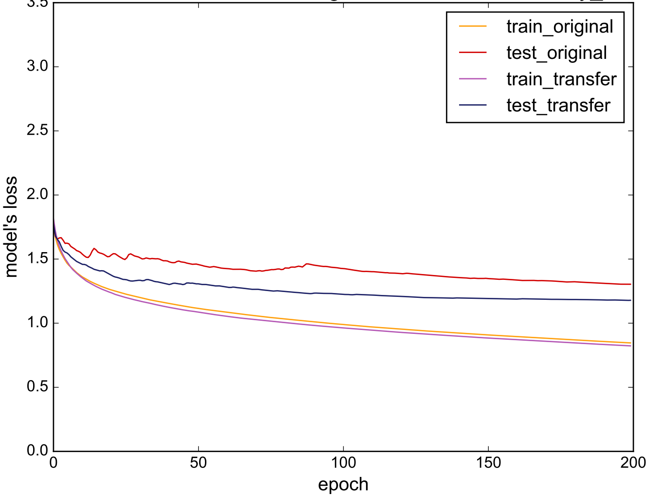
Source: BirdChicken - Target: uWaveGestureLibrary_Y
