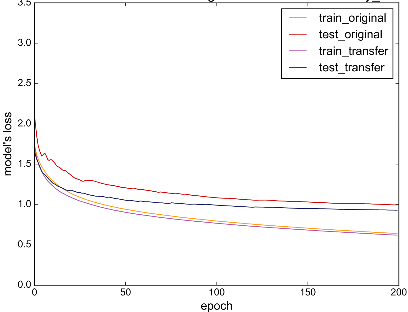
Source: BirdChicken - Target: uWaveGestureLibrary_Z
