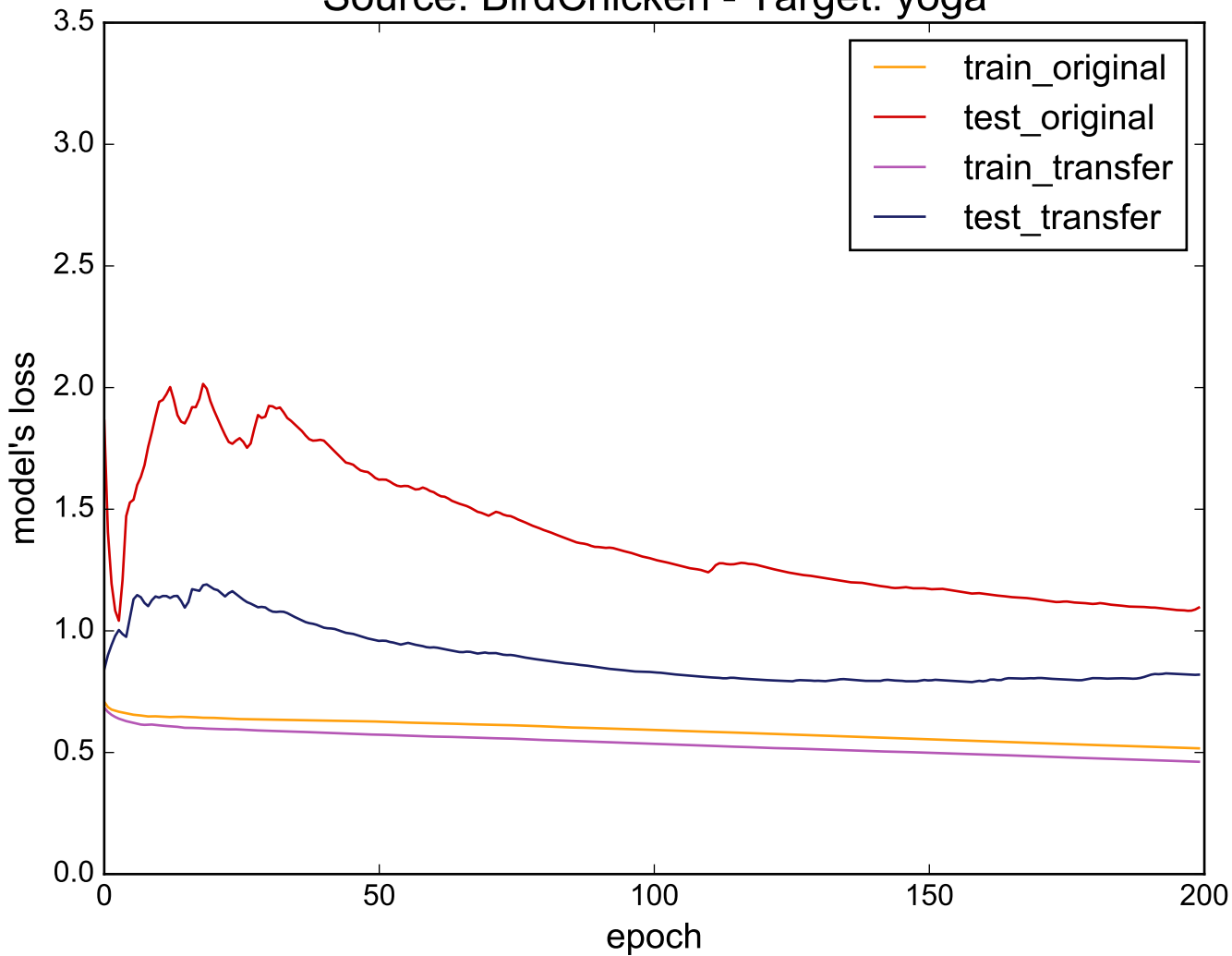
Source: BirdChicken - Target: yoga
