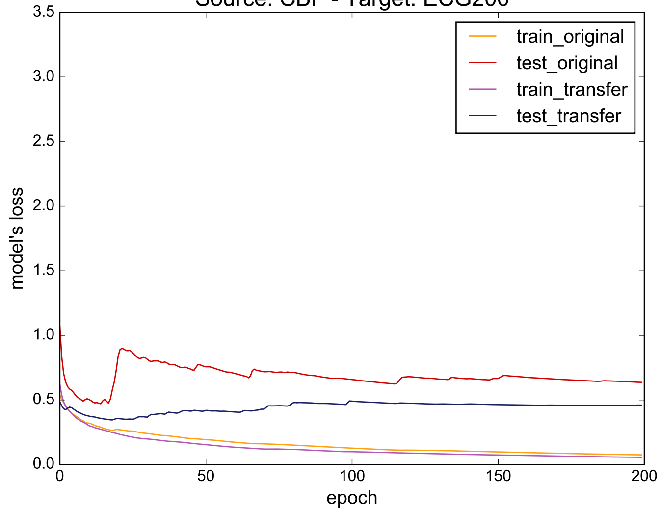
Source: CBF - Target: ECG200
