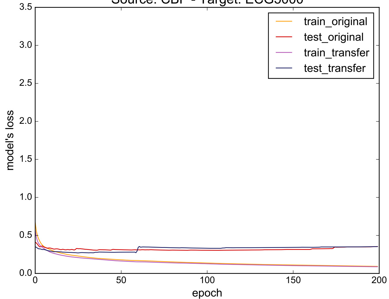
Source: CBF - Target: ECG5000
