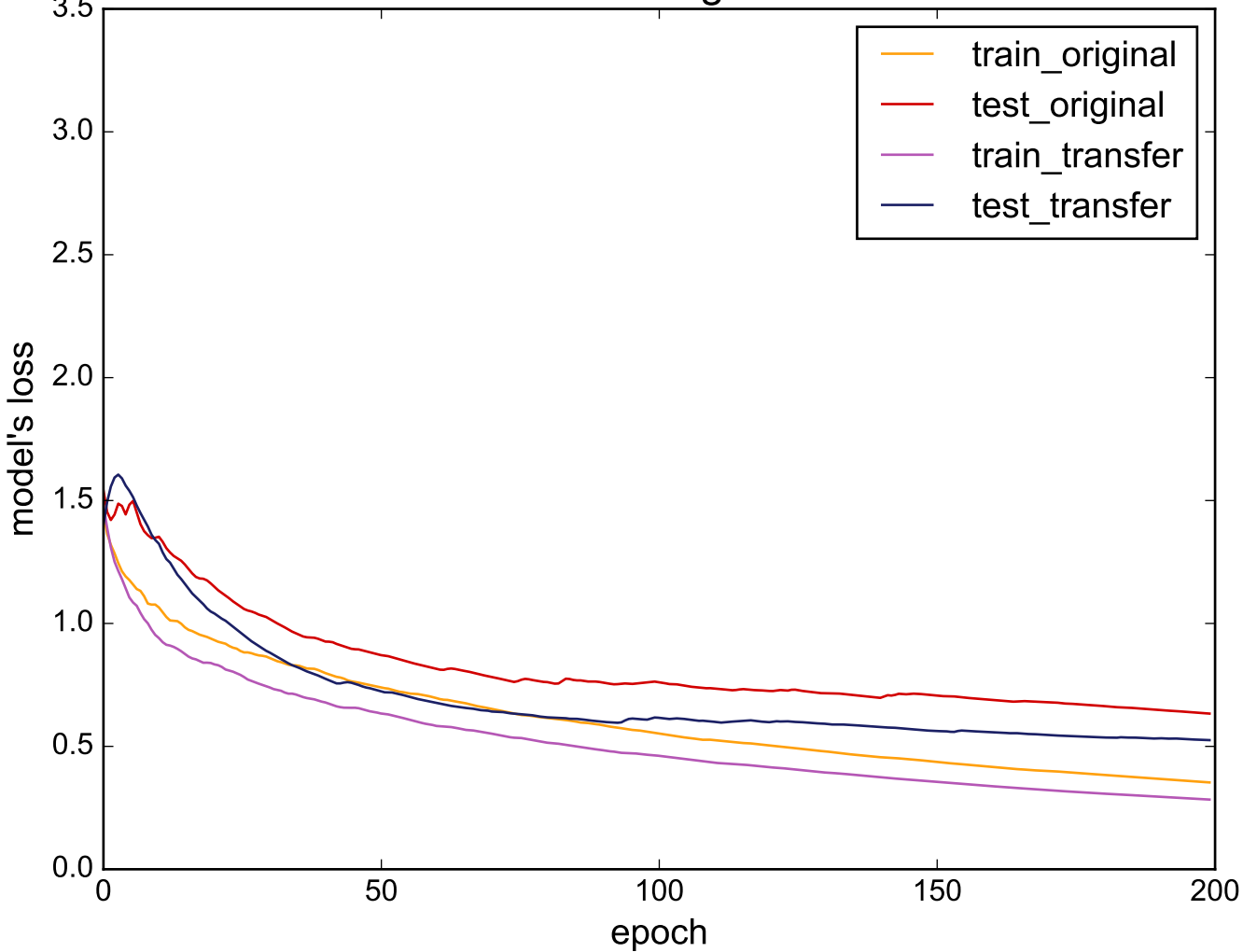
Source: CBF - Target: FaceFour
