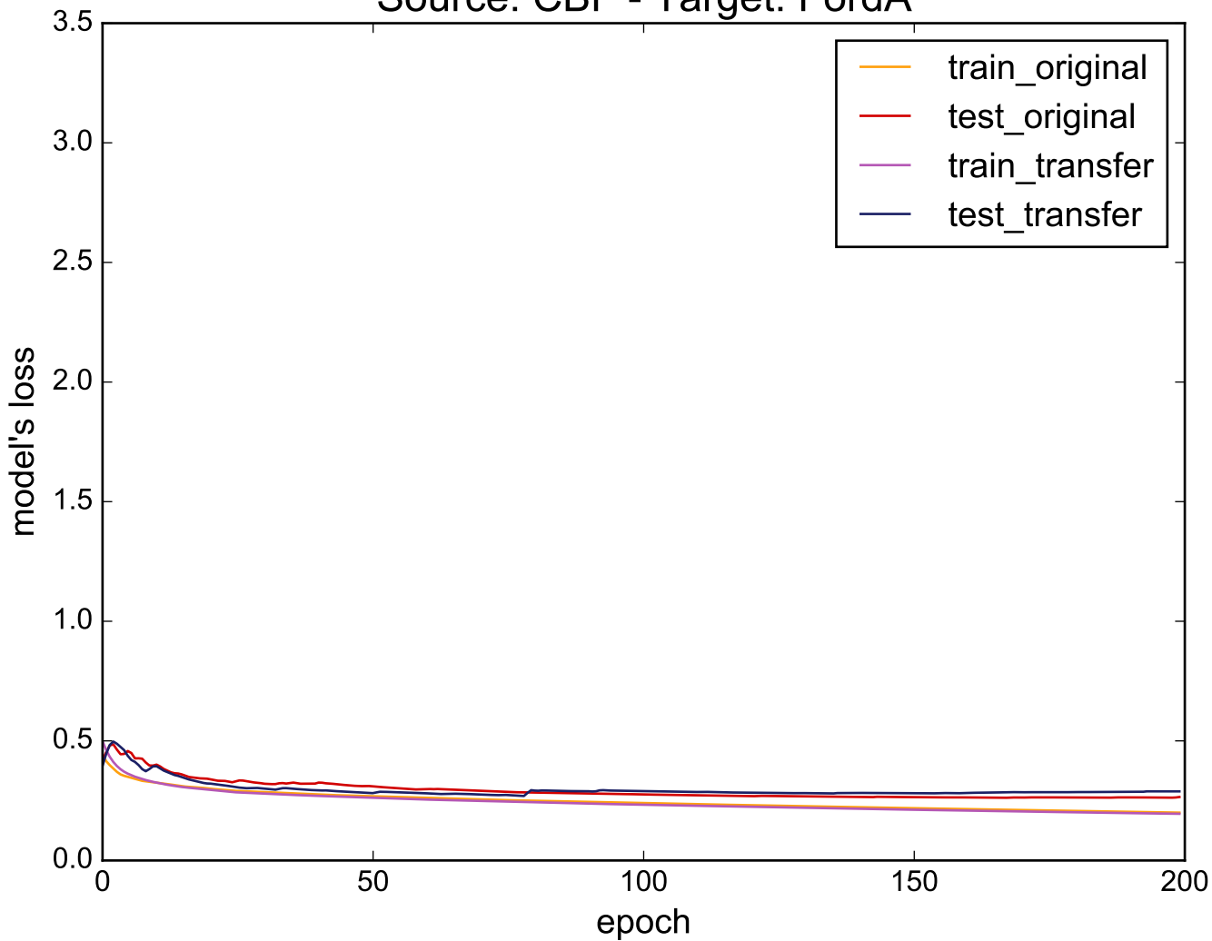
Source: CBF - Target: FordA
