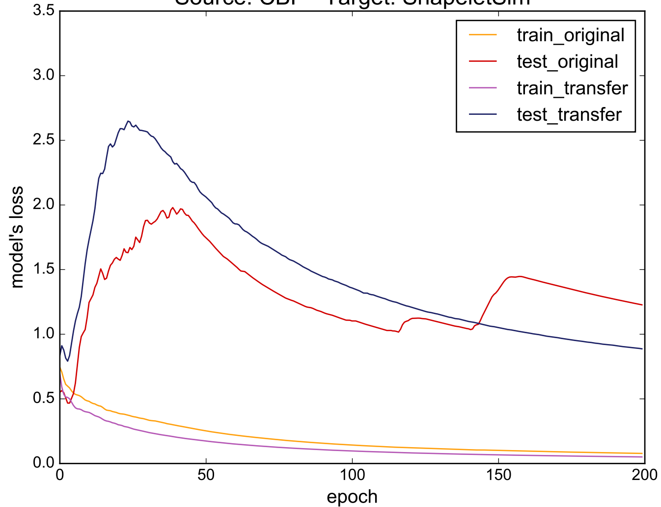
Source: CBF - Target: ShapeletSim
