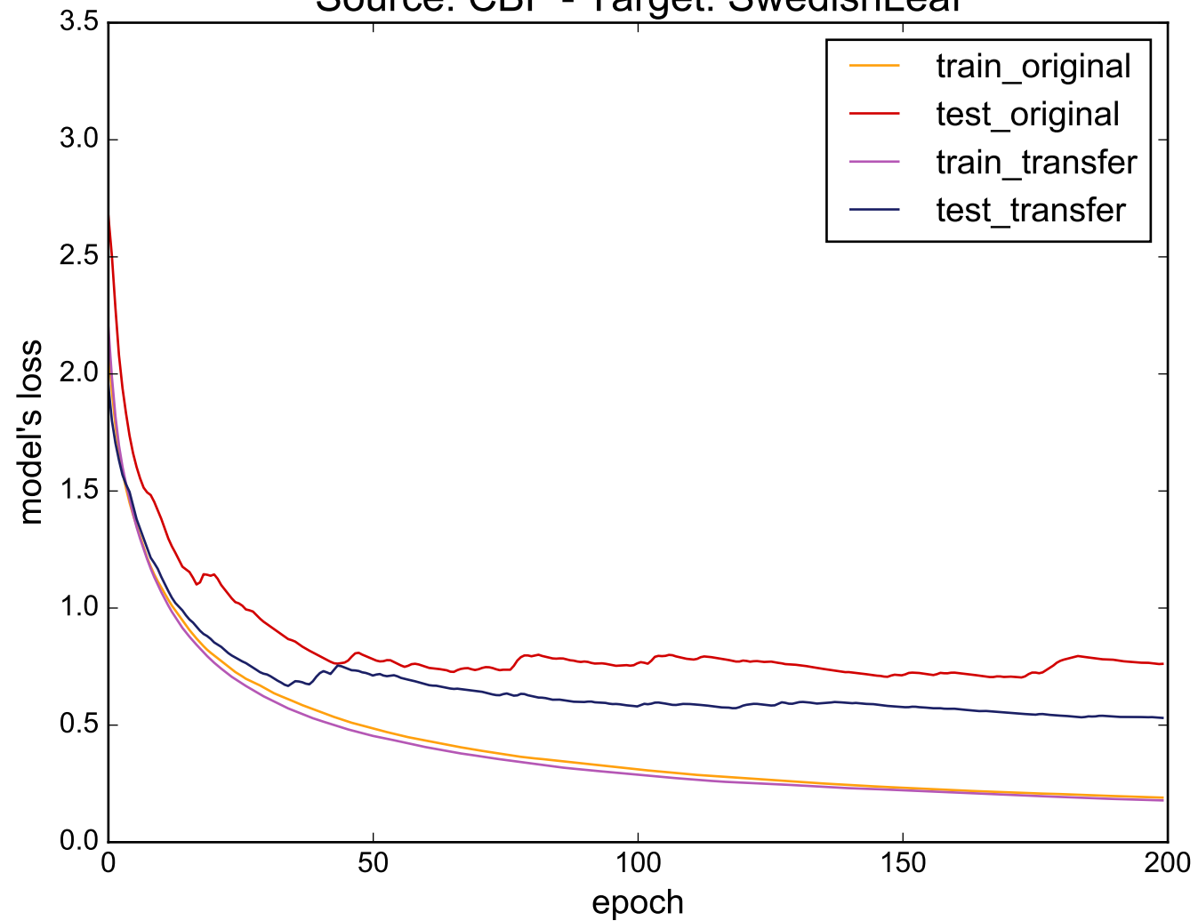
Source: CBF - Target: SwedishLeaf
