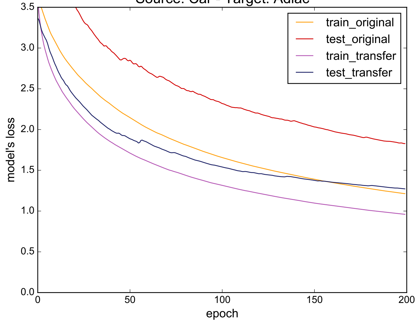
Source: Car - Target: Adiac
