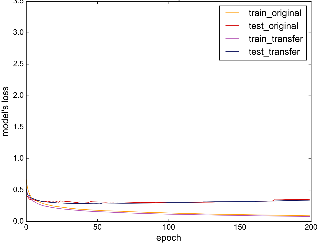
Source: Car - Target: ECG5000
