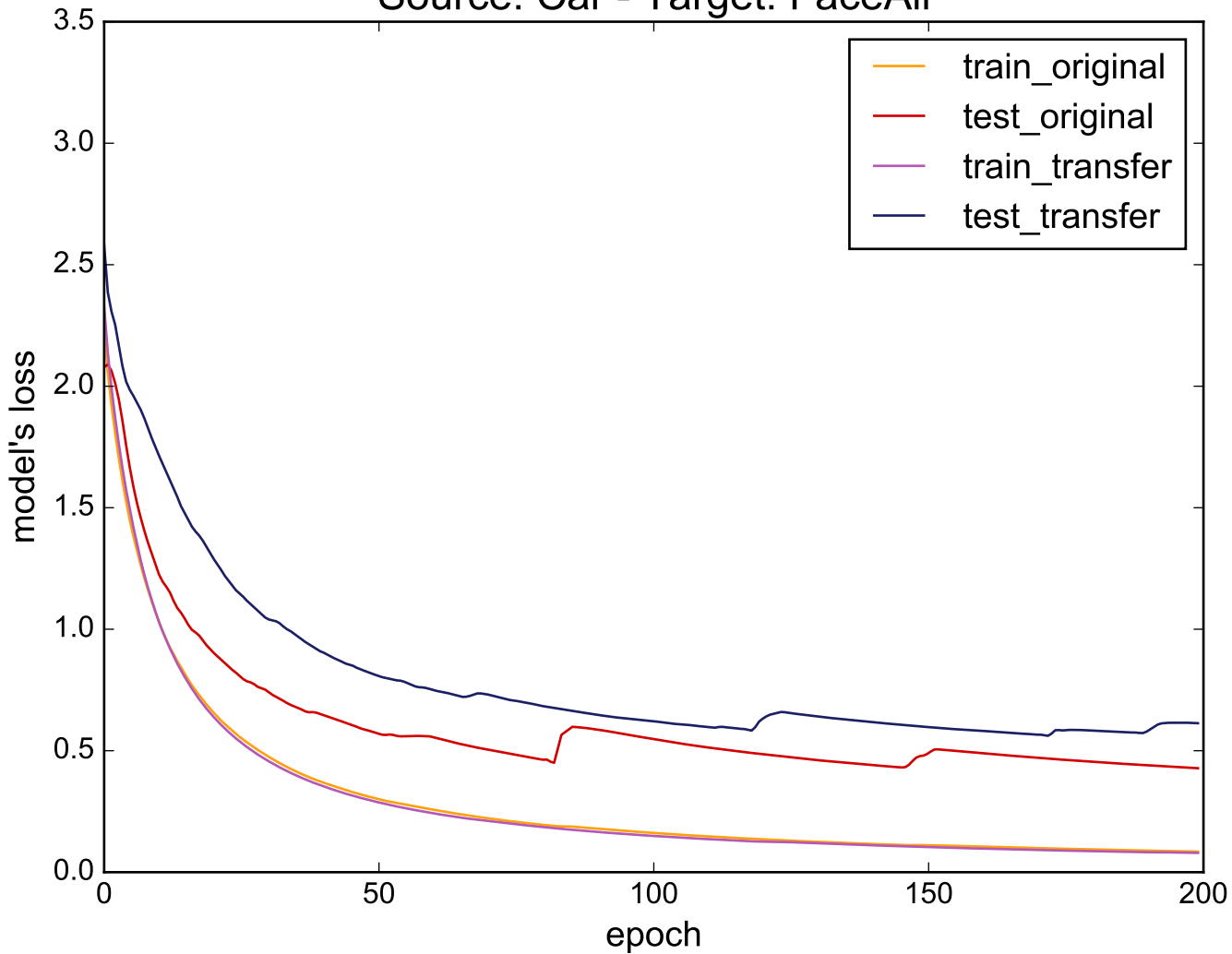
Source: Car - Target: FaceAll
