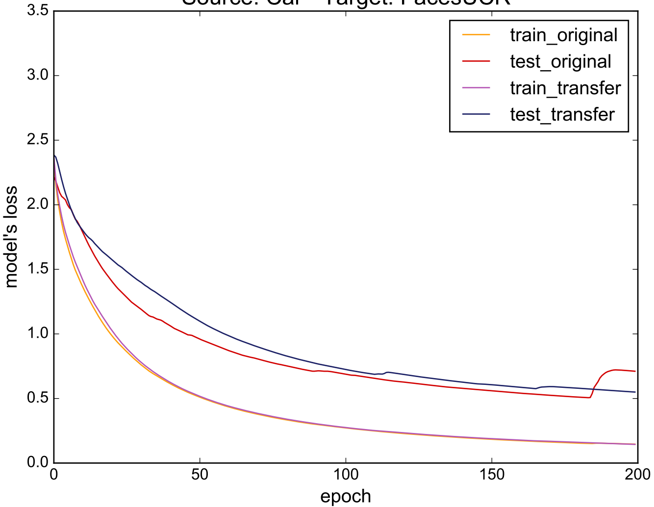
Source: Car - Target: FacesUCR
