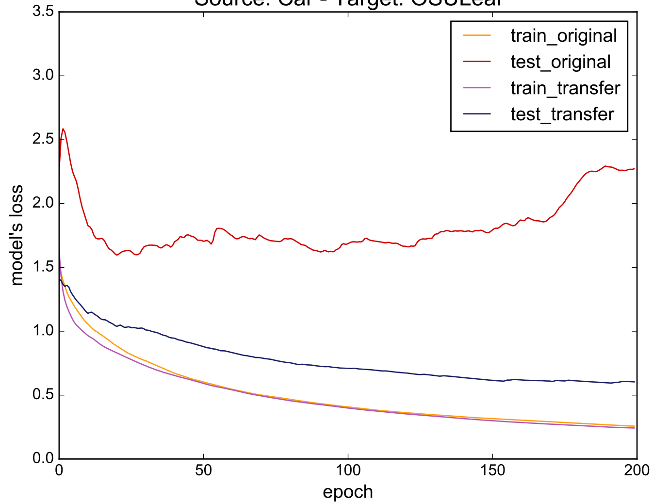
Source: Car - Target: OSULeaf
