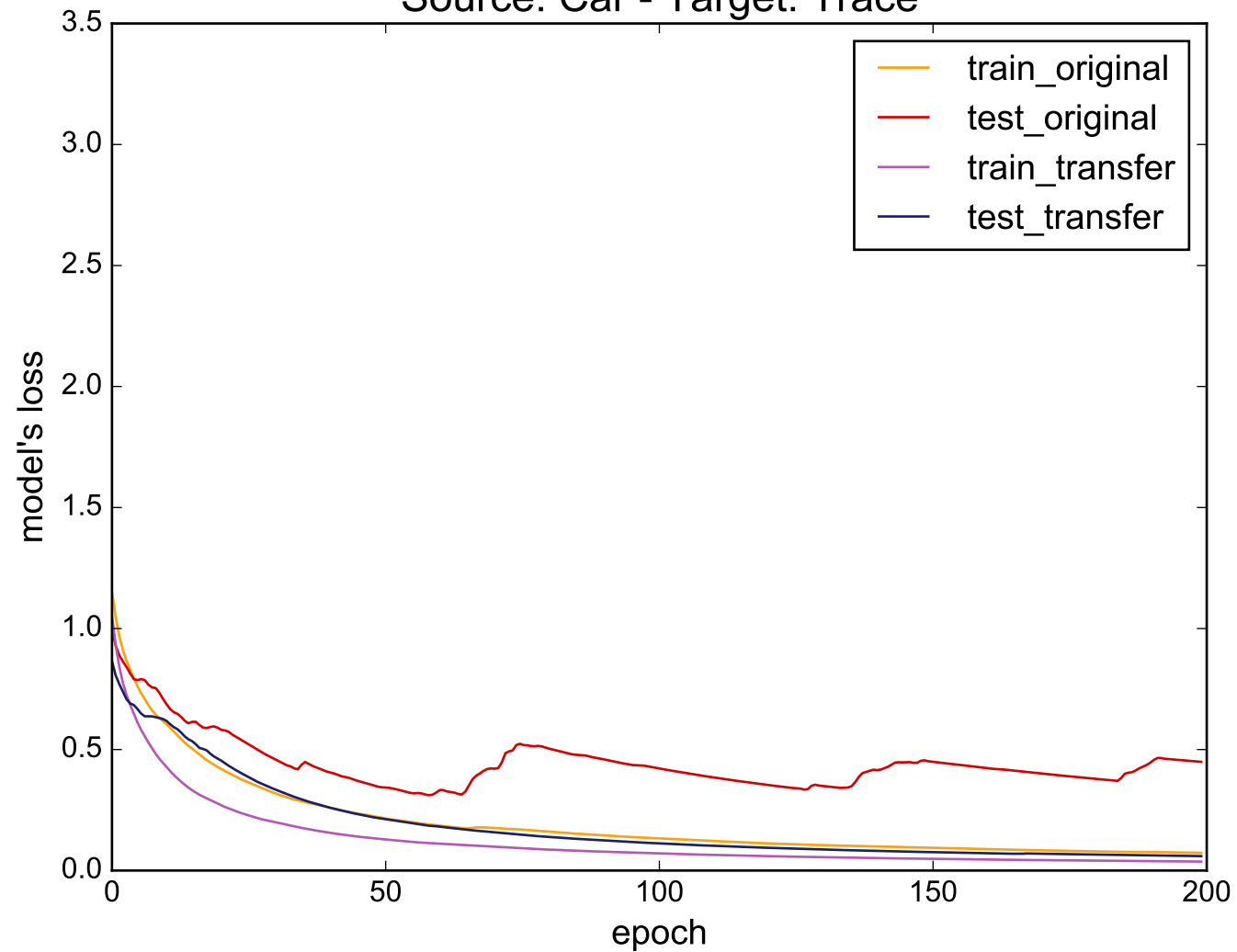
Source: Car - Target: Trace
