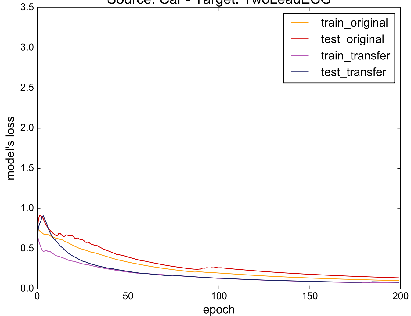
Source: Car - Target: TwoLeadECG
