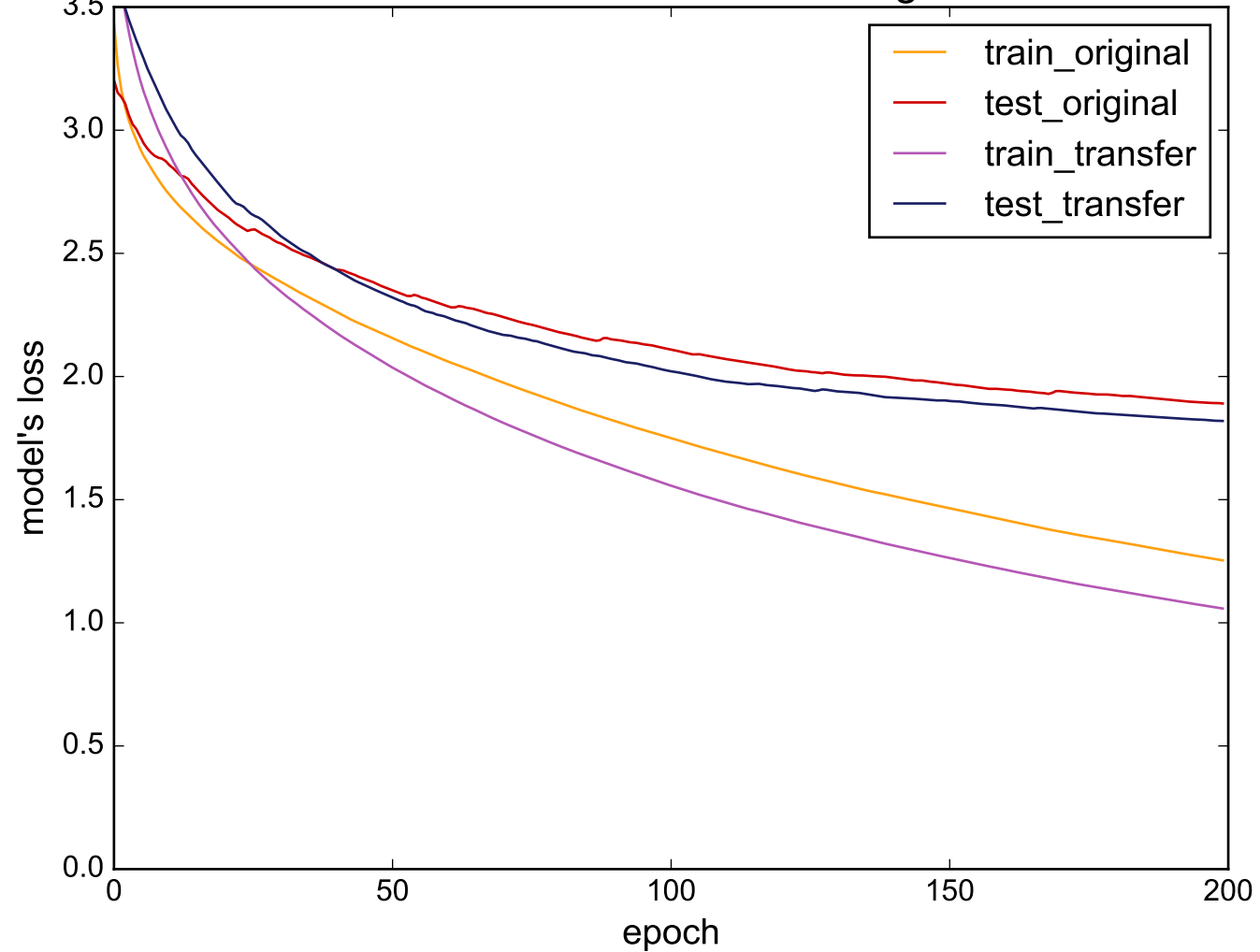
Source: ChlorineConcentration - Target: 50words
