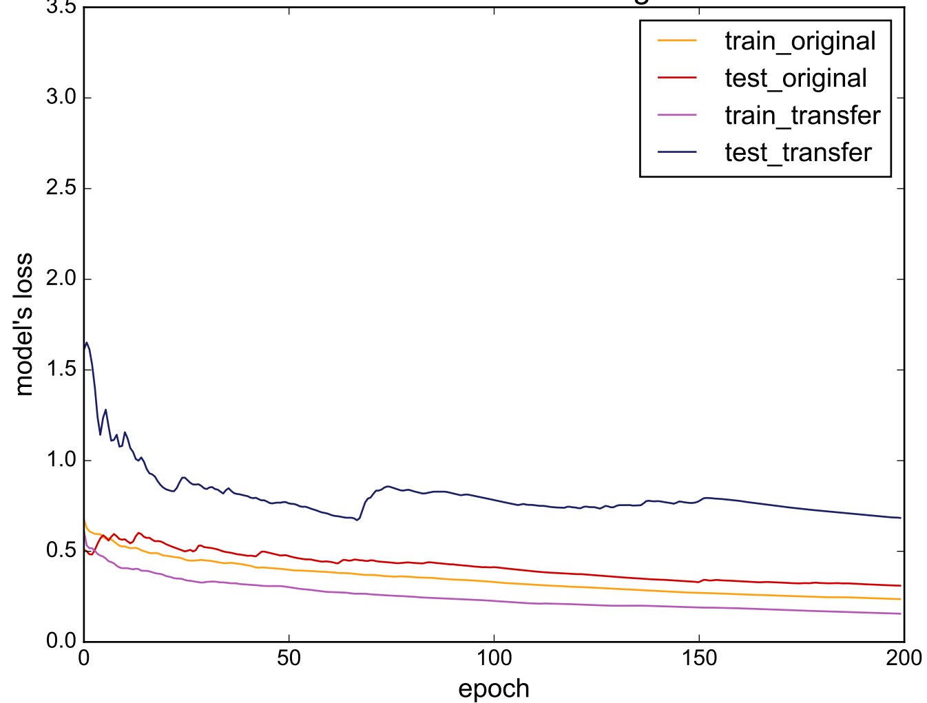
Source: ChlorineConcentration - Target: BirdChicken
