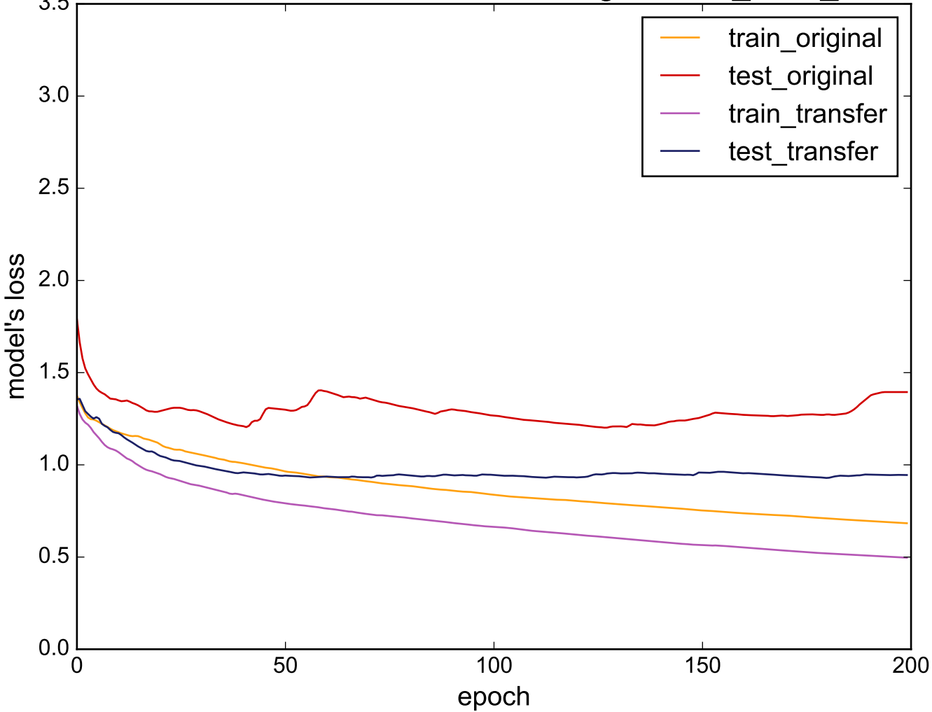
Source: ChlorineConcentration - Target: CinC_ECG_torso
