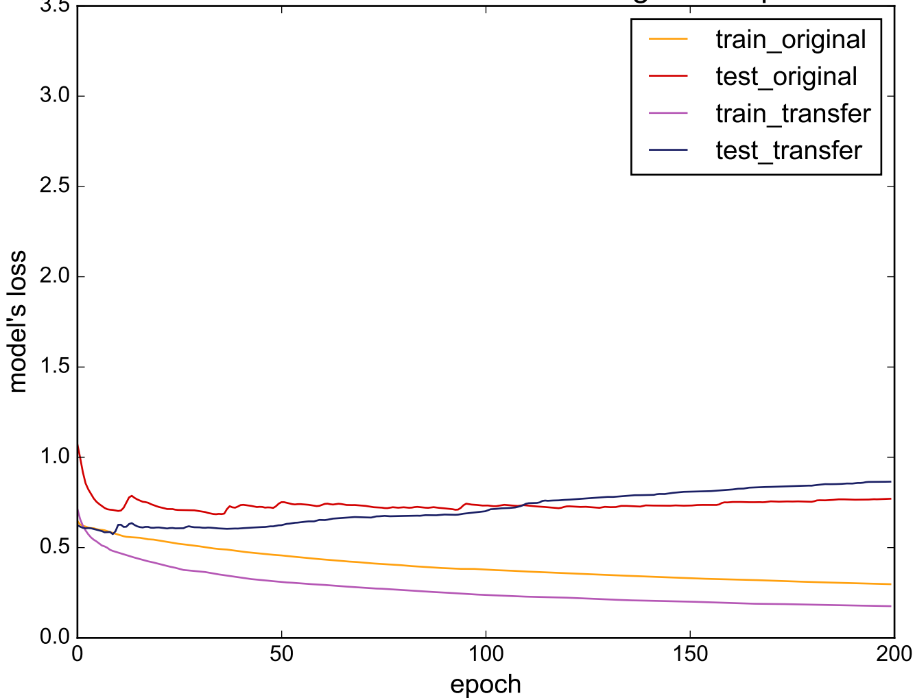
Source: ChlorineConcentration - Target: Computers
