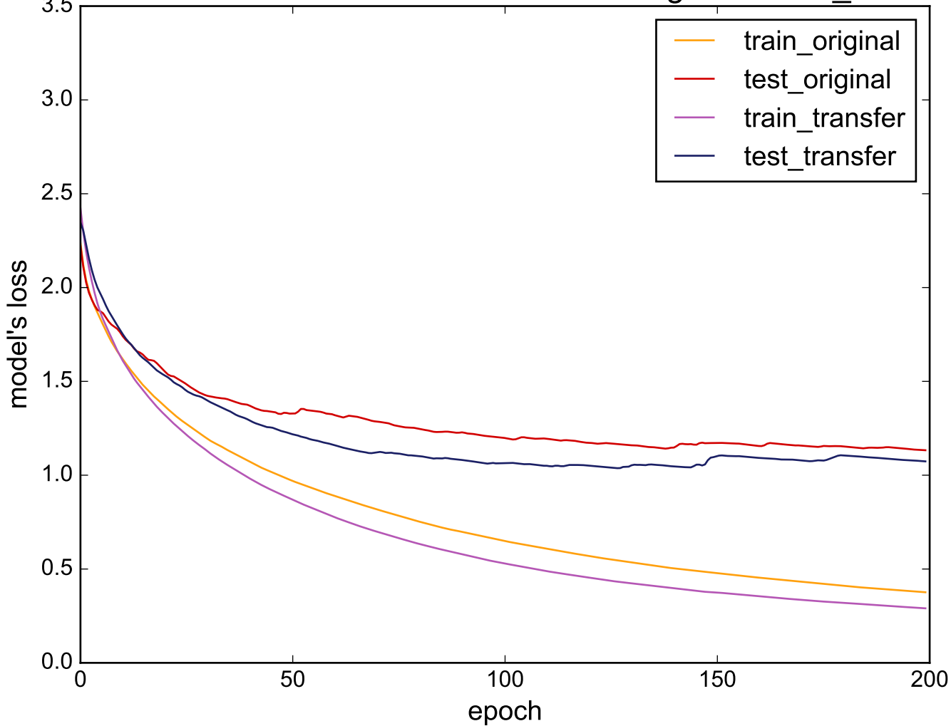
Source: ChlorineConcentration - Target: Cricket_Y
