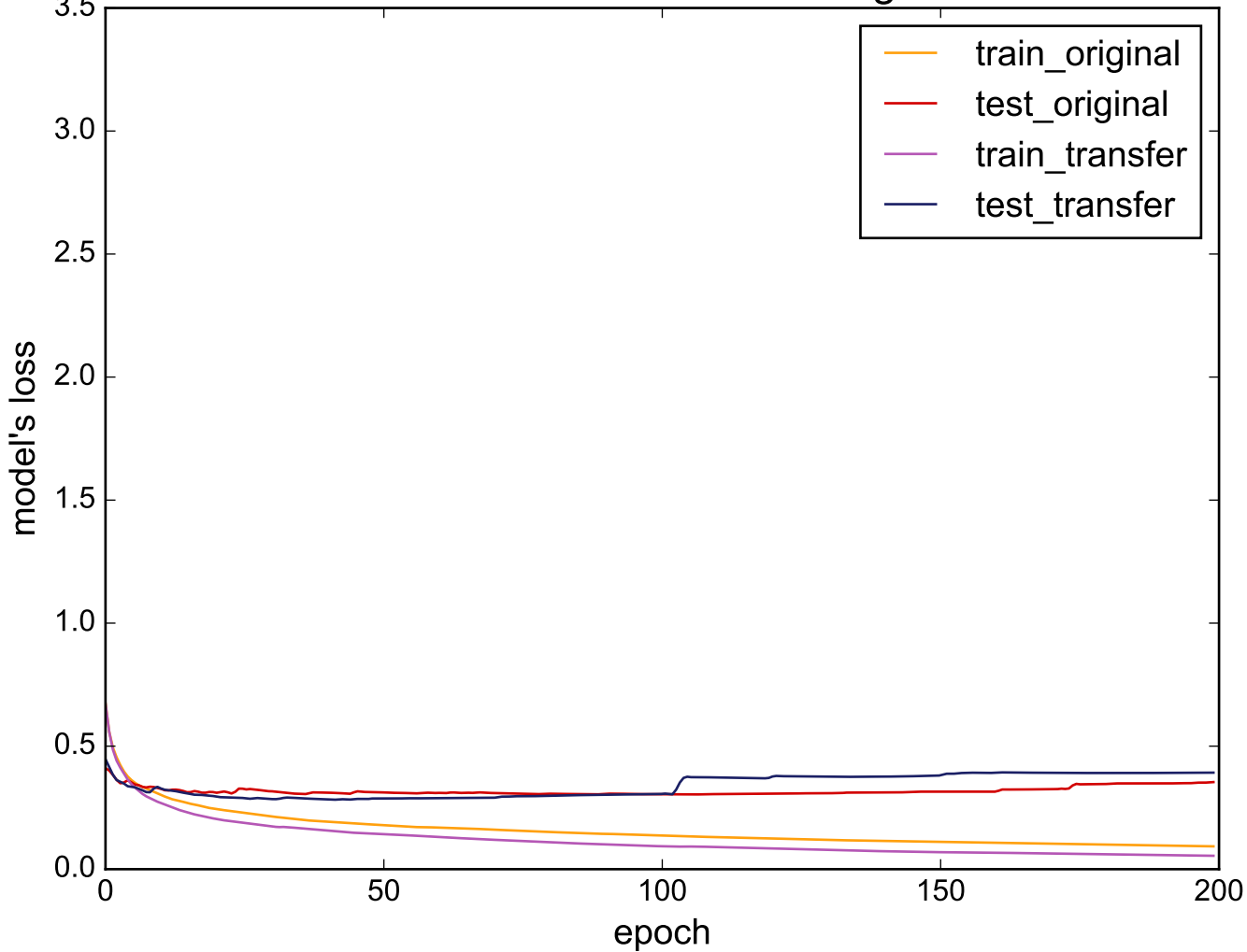
Source: ChlorineConcentration - Target: ECG5000
