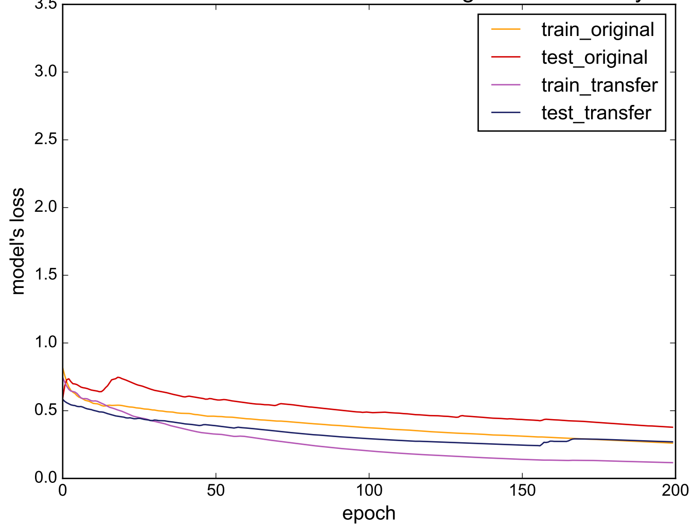
Source: ChlorineConcentration - Target: ECGFiveDays
