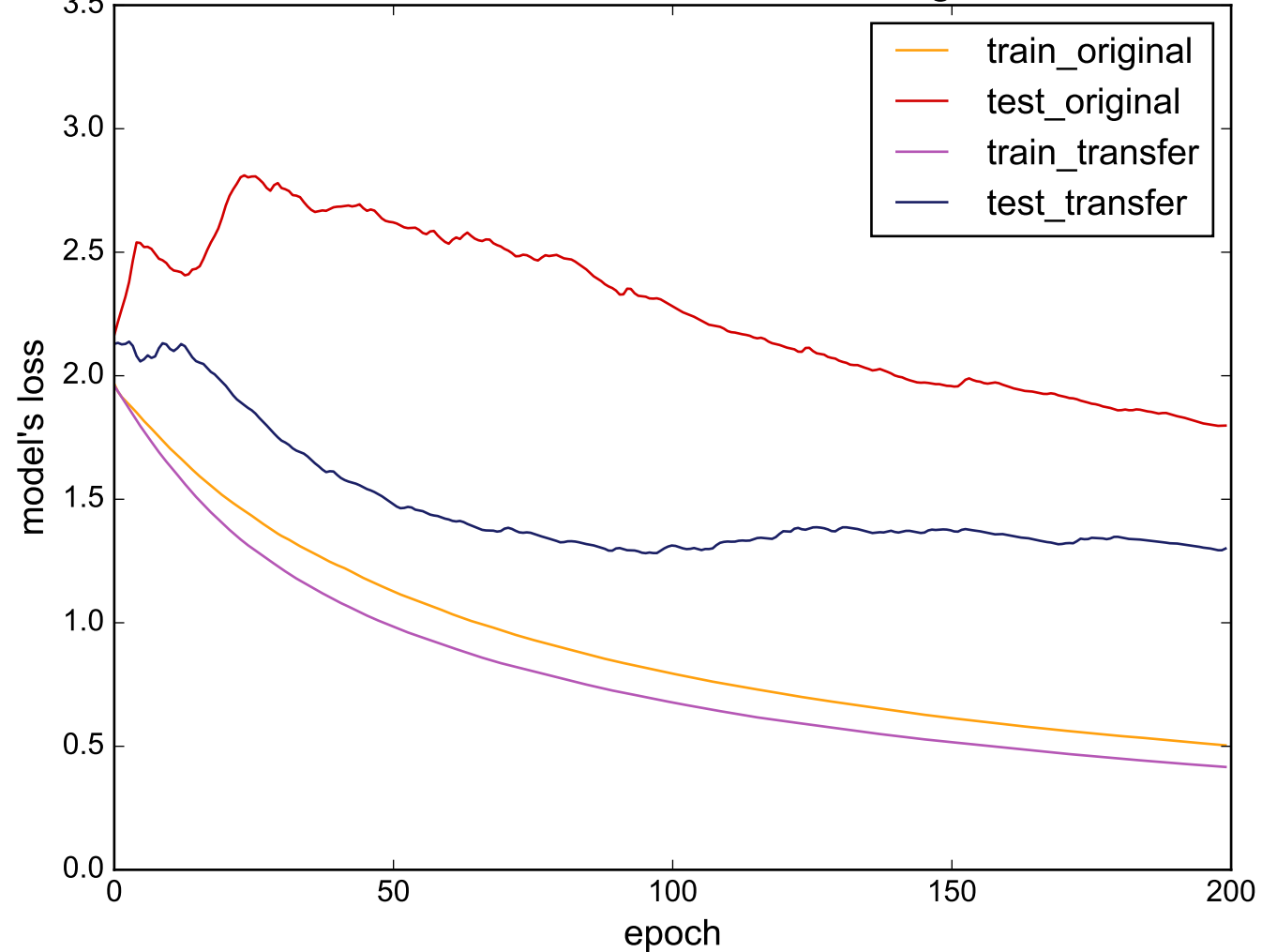
Source: ChlorineConcentration - Target: FISH
