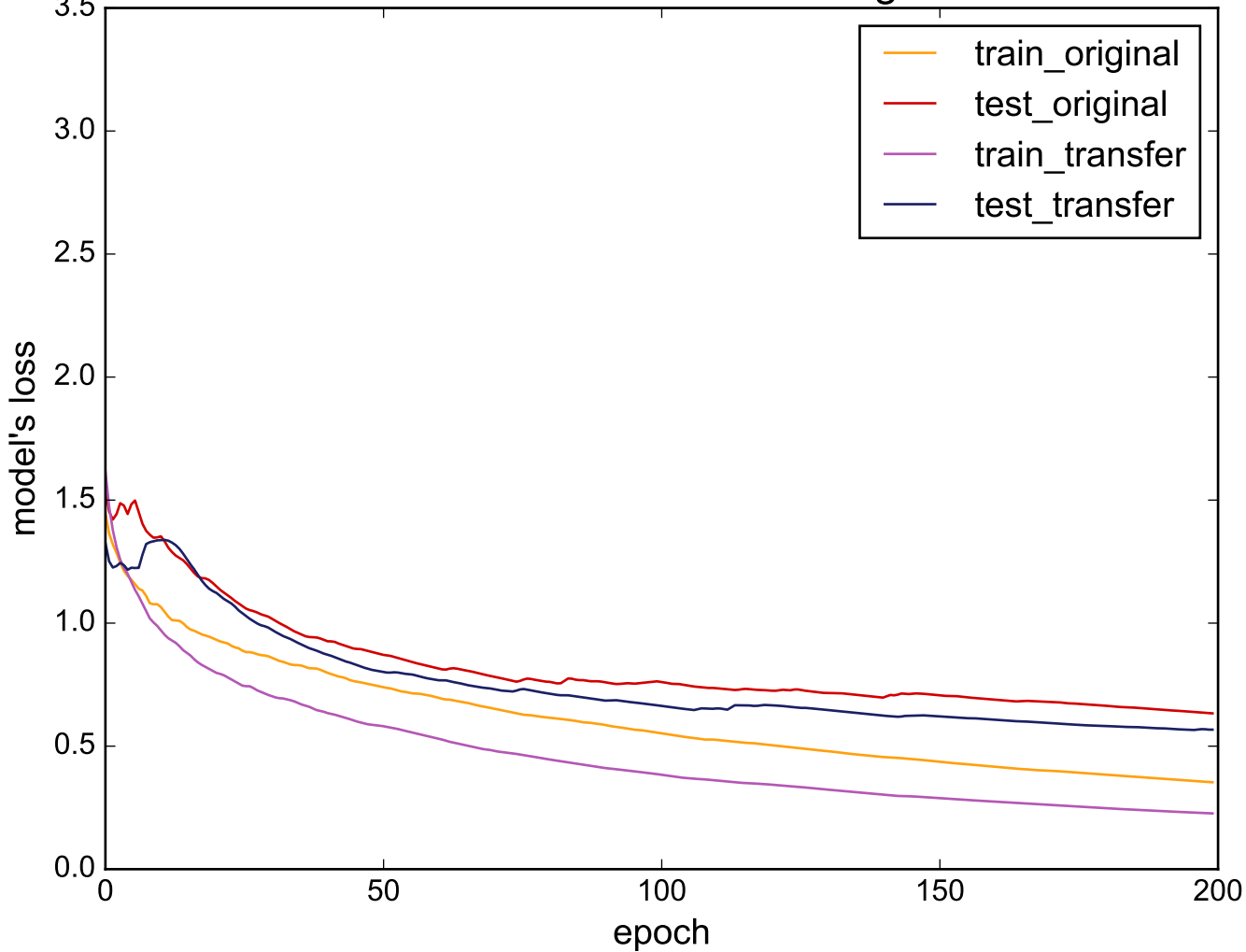
Source: ChlorineConcentration - Target: FaceFour
