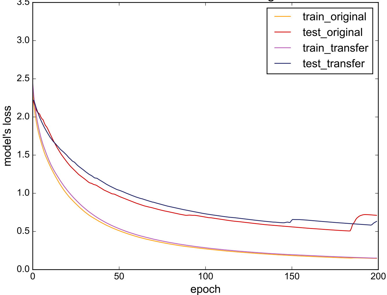
Source: ChlorineConcentration - Target: FacesUCR
