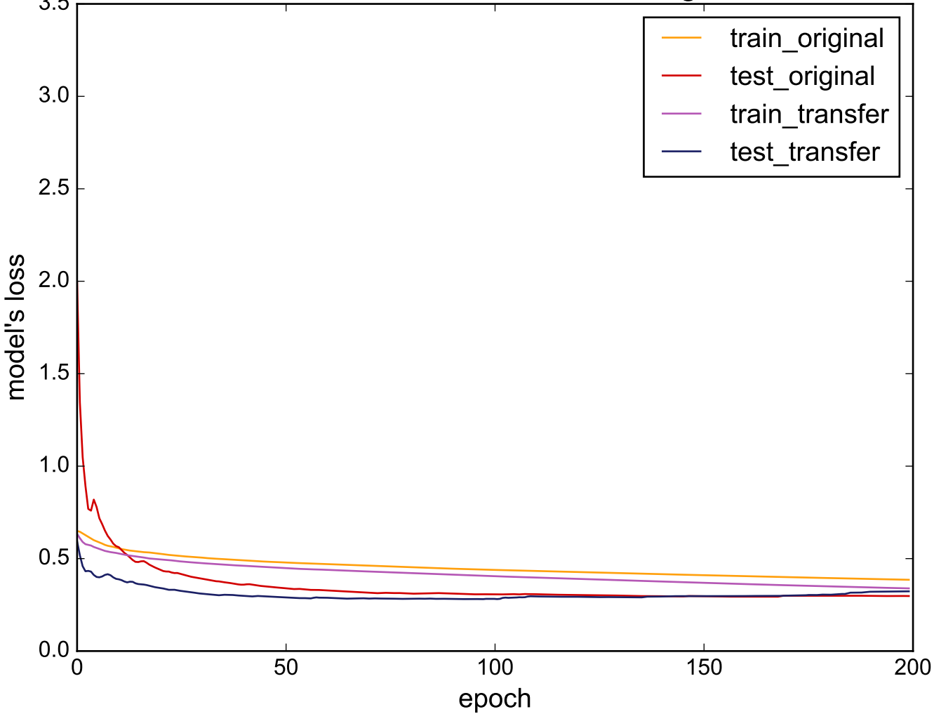
Source: ChlorineConcentration - Target: FordB
