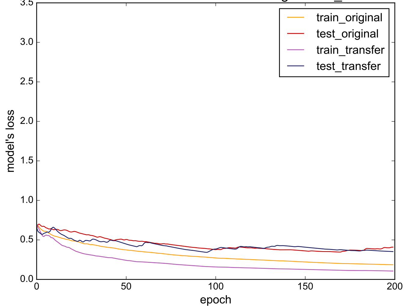
Source: ChlorineConcentration - Target: Gun_Point
