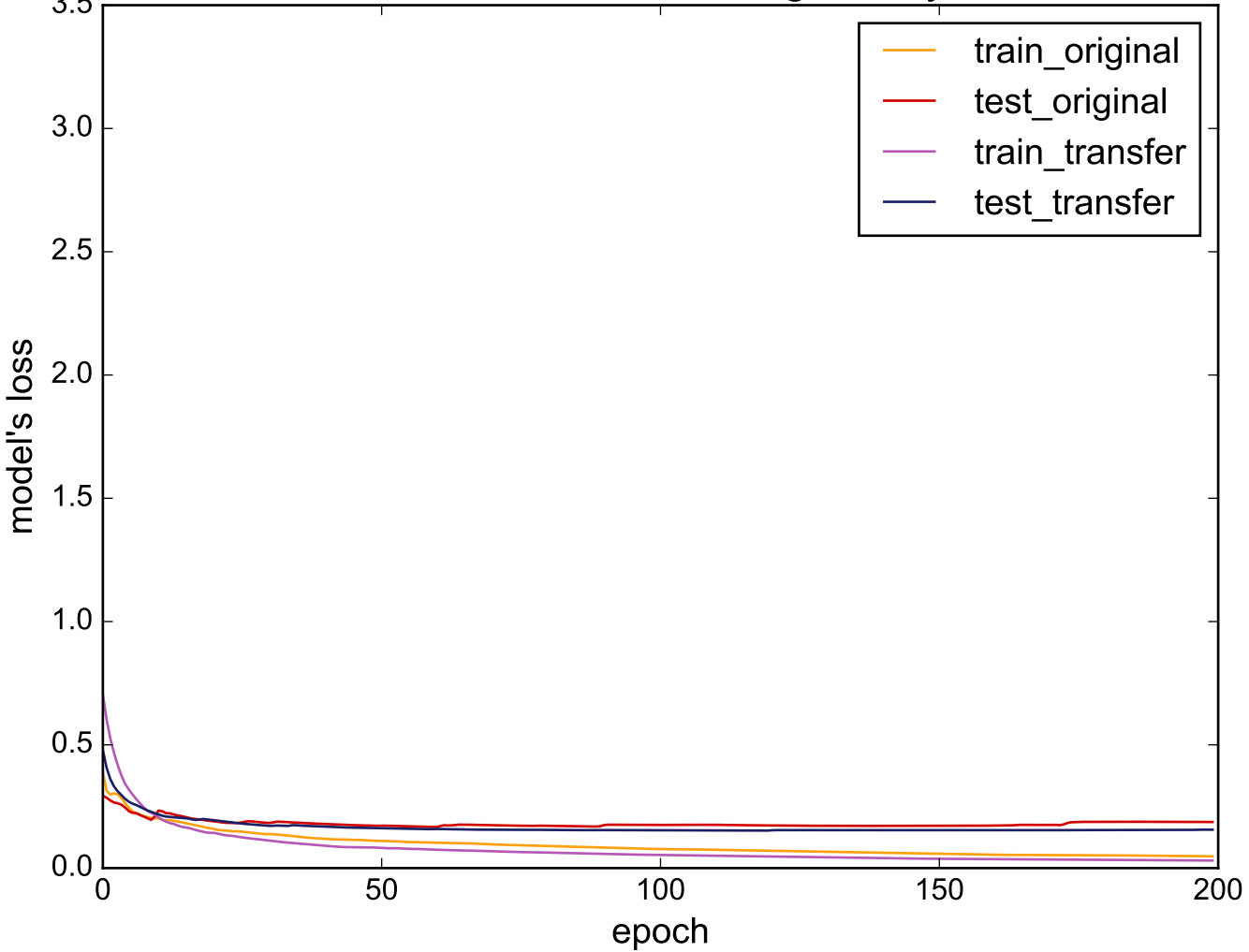
Source: ChlorineConcentration - Target: ItalyPowerDemand
