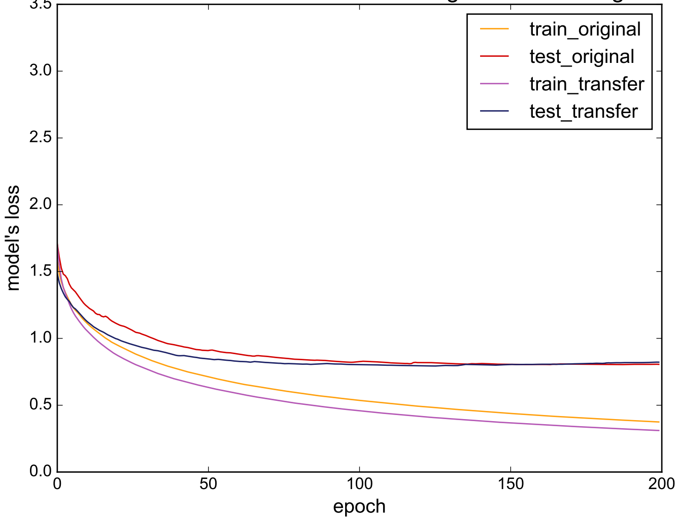
Source: ChlorineConcentration - Target: MedicalImages
