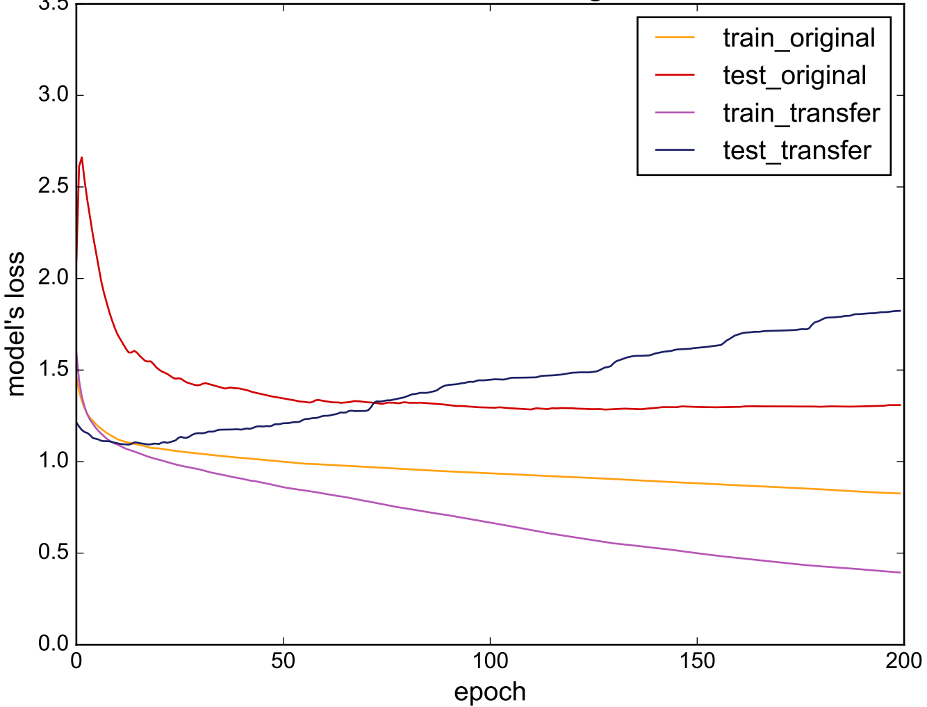
Source: ChlorineConcentration - Target: MiddlePhalanxTW
