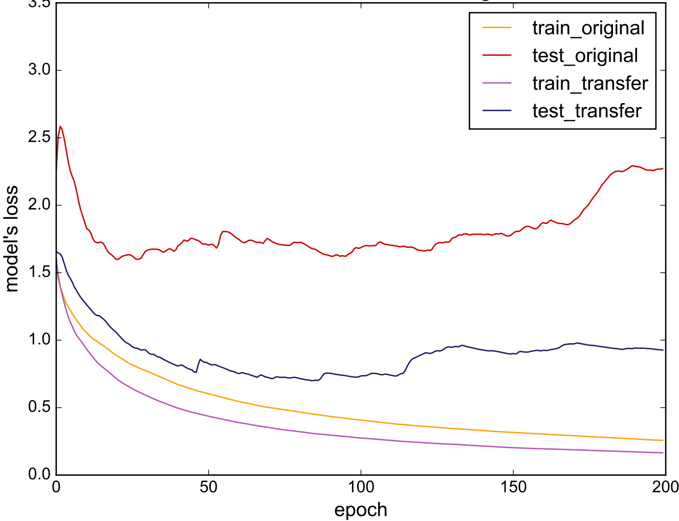
Source: ChlorineConcentration - Target: OSULeaf
