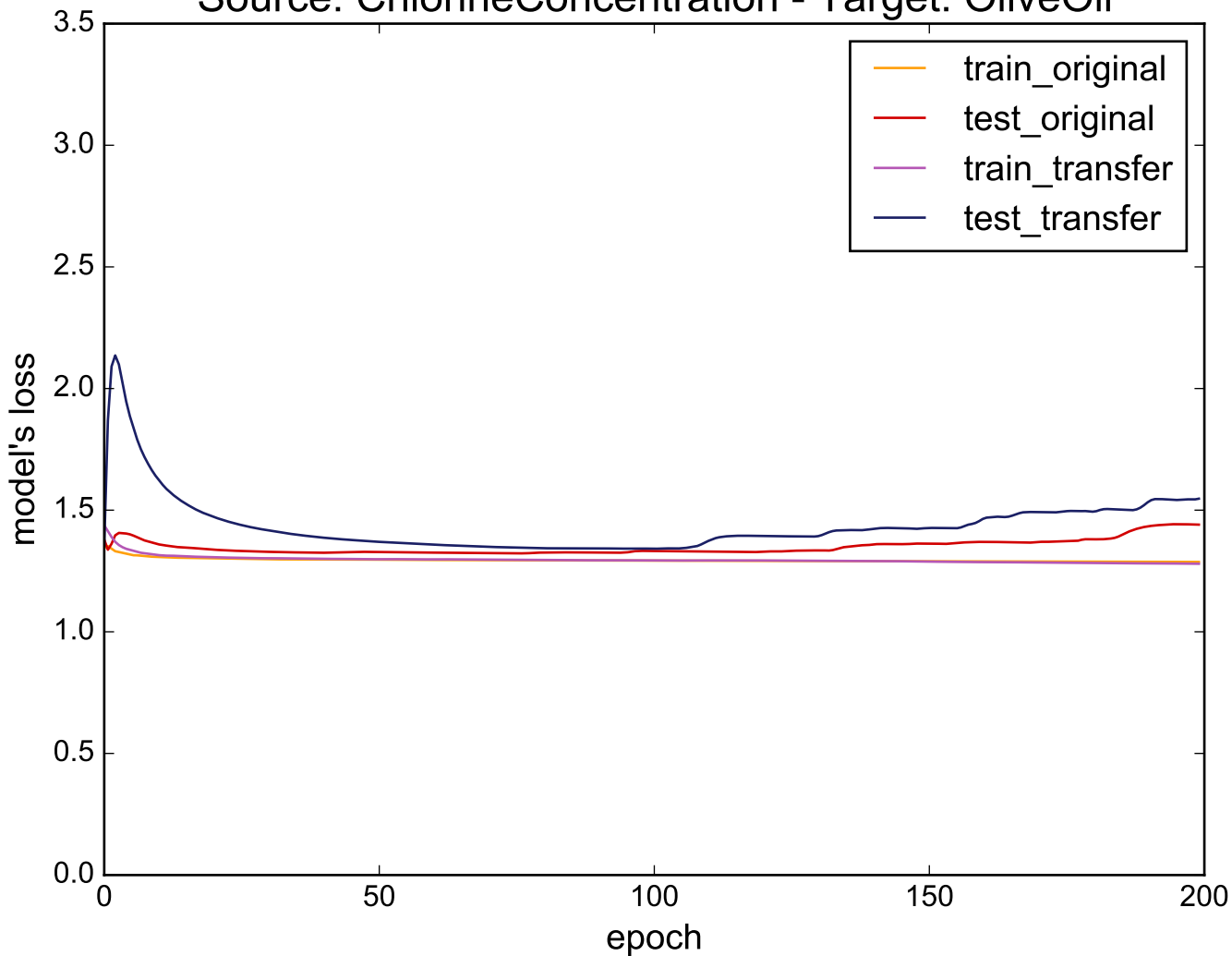
Source: ChlorineConcentration - Target: OliveOil
