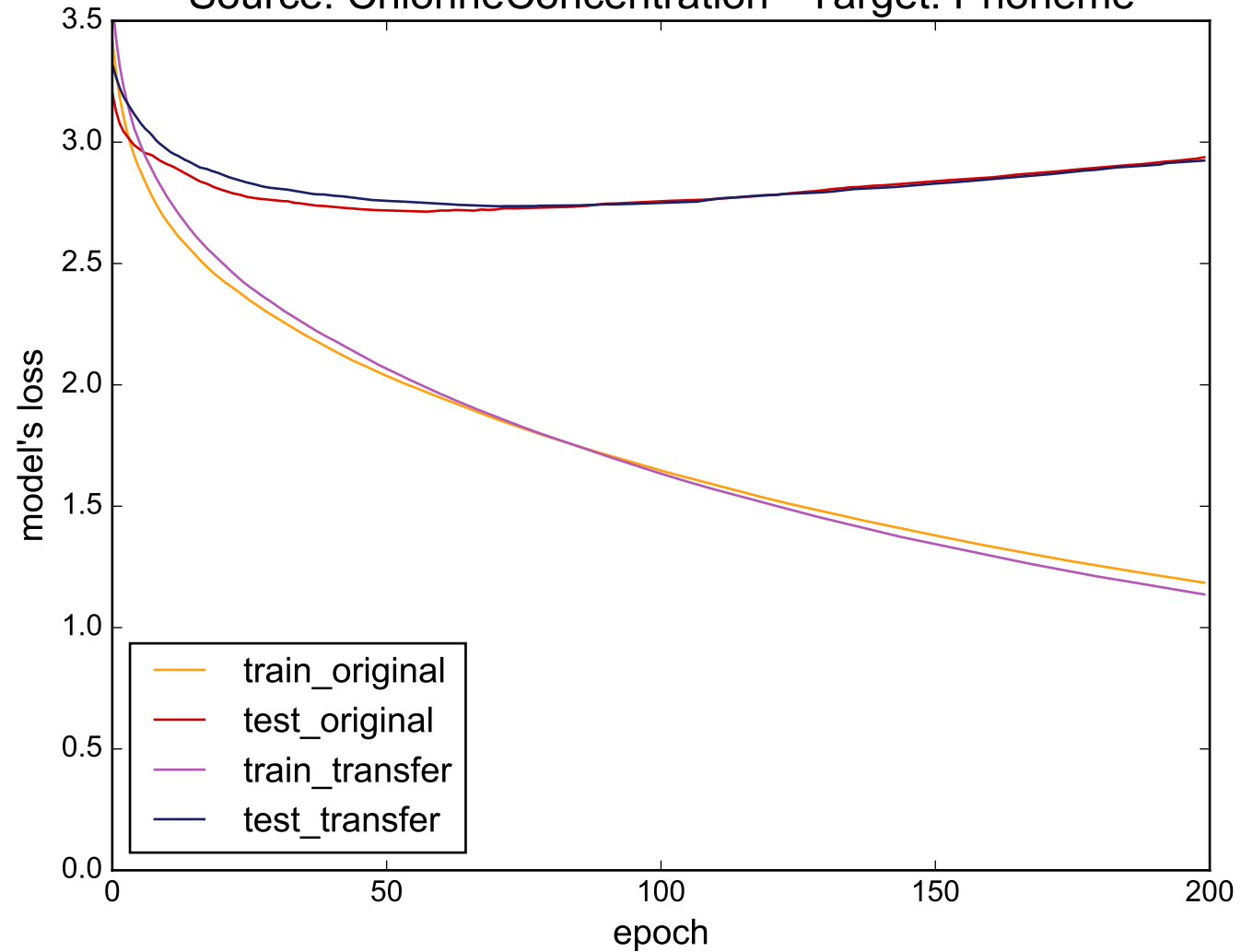
Source: ChlorineConcentration - Target: Phoneme
