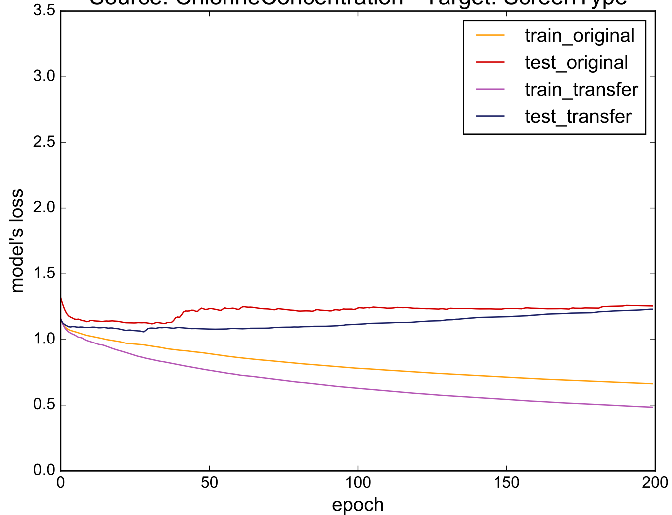
Source: ChlorineConcentration - Target: ScreenType
