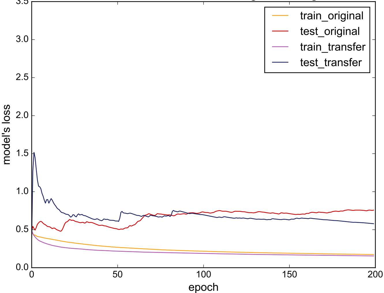
Source: ChlorineConcentration - Target: StarLightCurves
