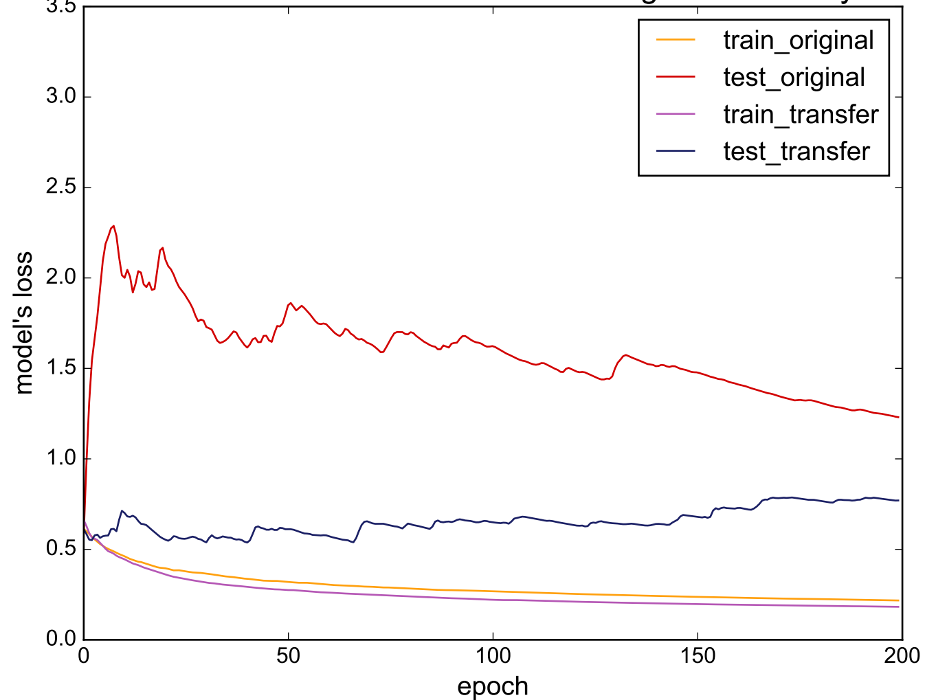
Source: ChlorineConcentration - Target: Strawberry
