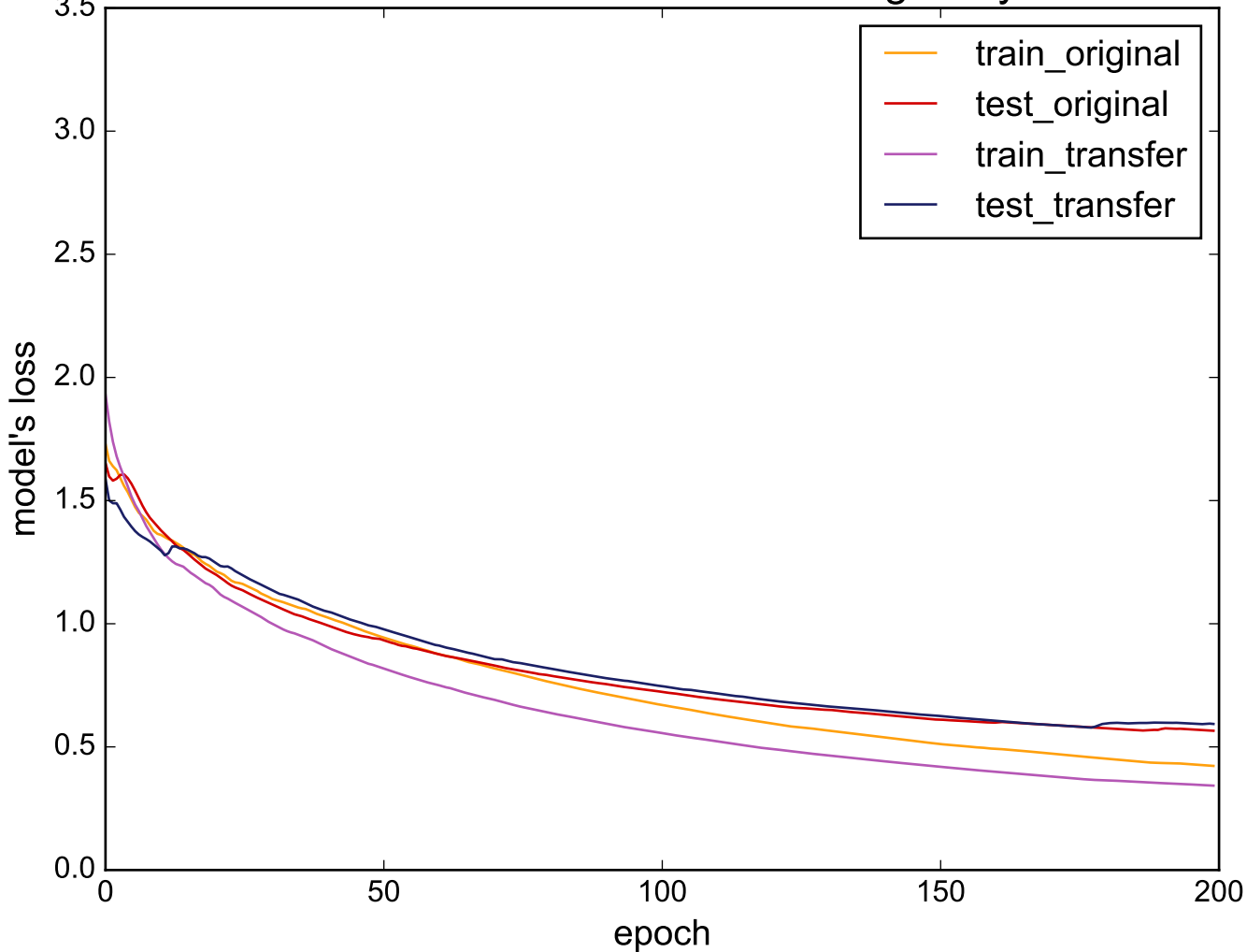
Source: ChlorineConcentration - Target: Symbols
